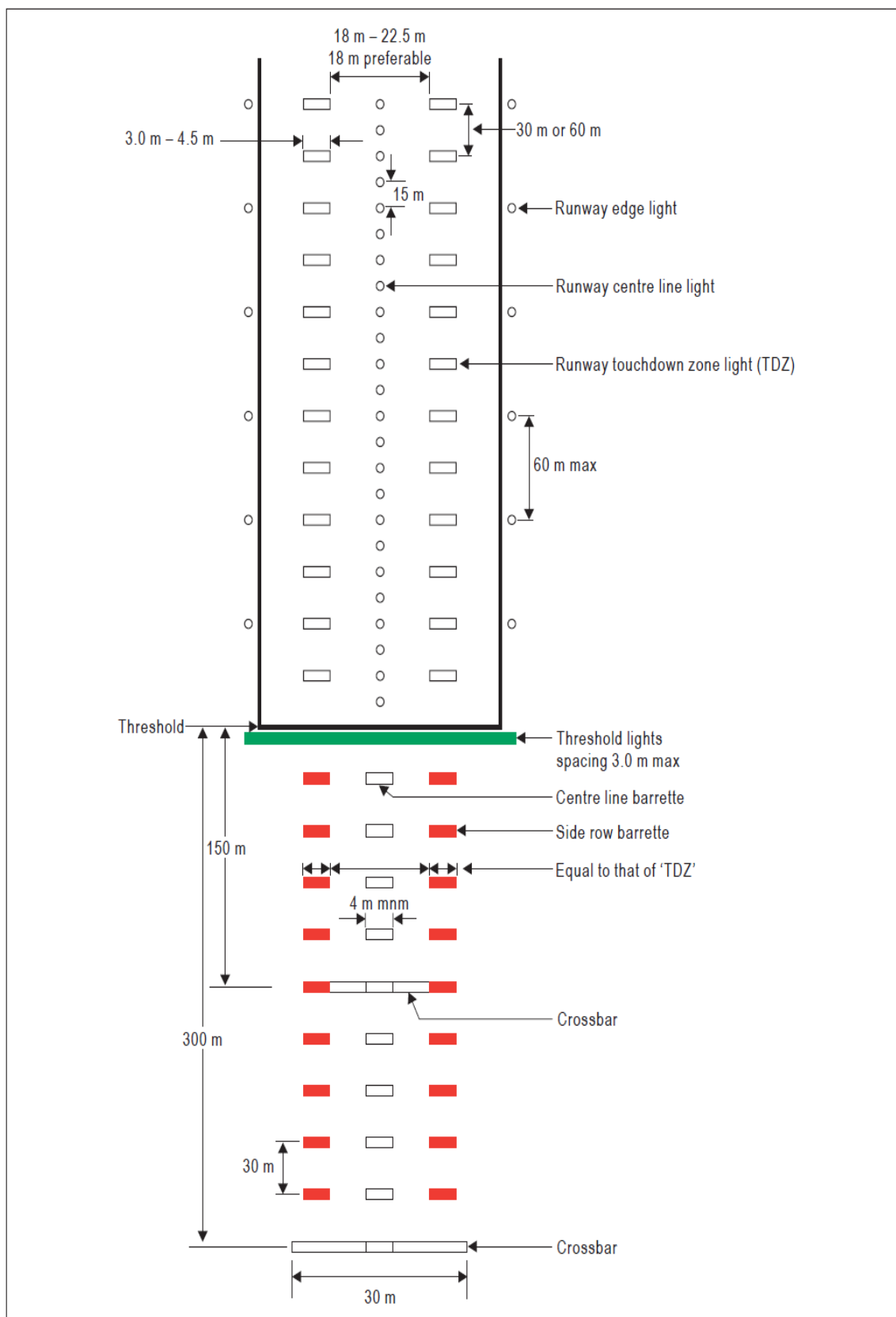
Figure 5-14. Inner 300 m approach and runway lighting for precision approach runways, categories II and III
