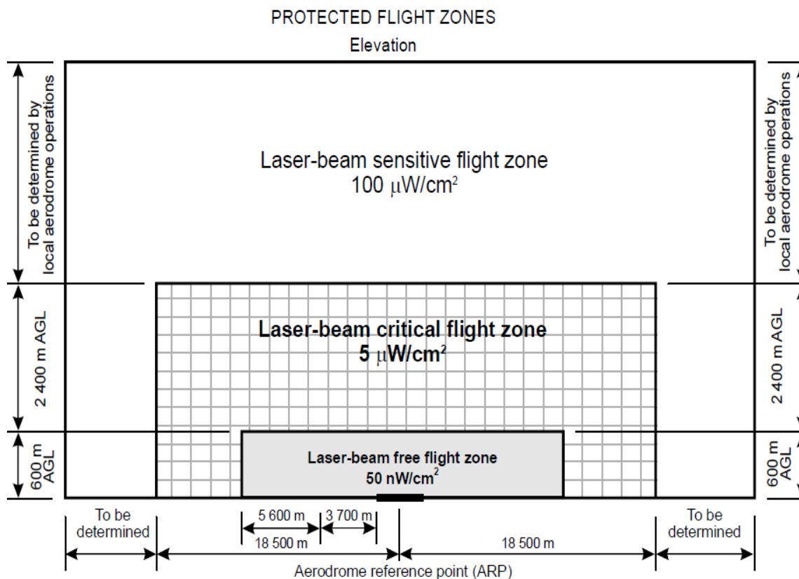
Figure 5-13. Protected flight zones with indication of maximum irradiance levels for visible laser beams
