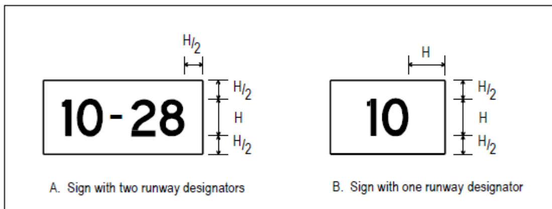
Figure A4-4. Sign dimensions
