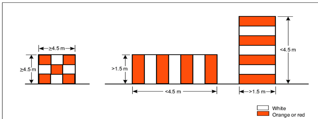
Figure 6-1. Basic marking patterns
