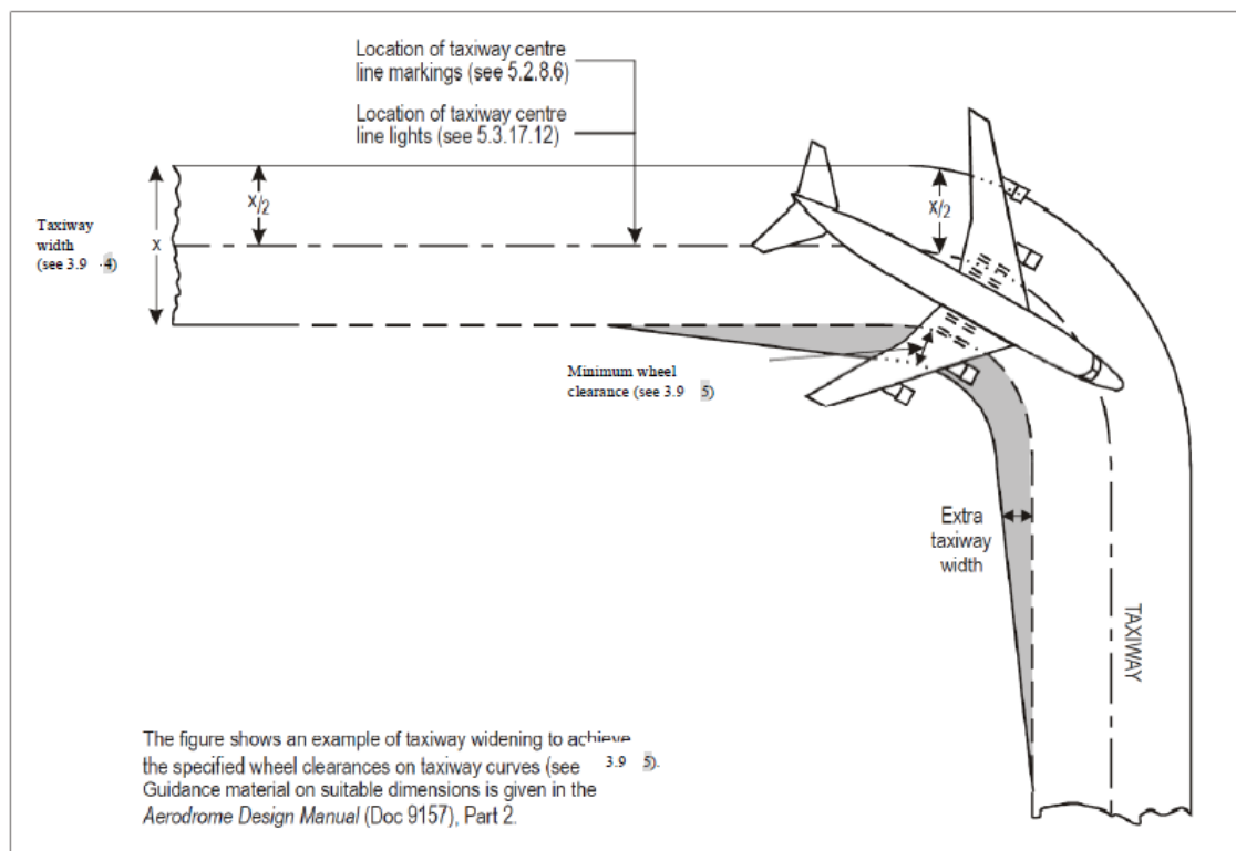
Figure 3-2. Taxiway Curve
