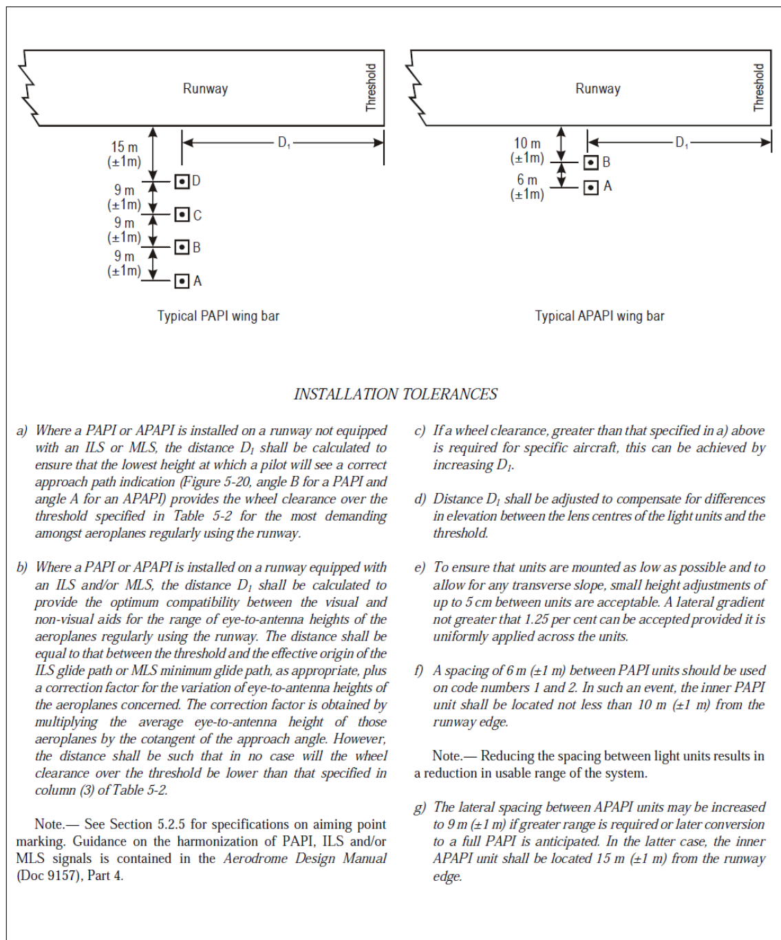
Figure 5-19. Siting of PAPI and APAPI
