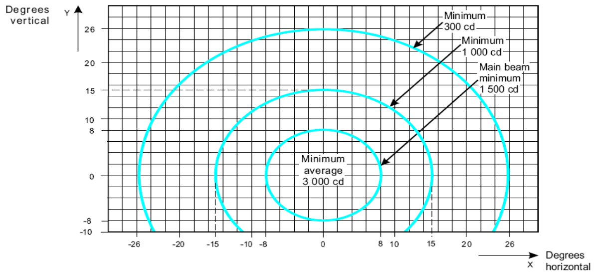
Figure A2-24. Isocandela diagram for each light in low-intensity runway guard lights, Configuration A
