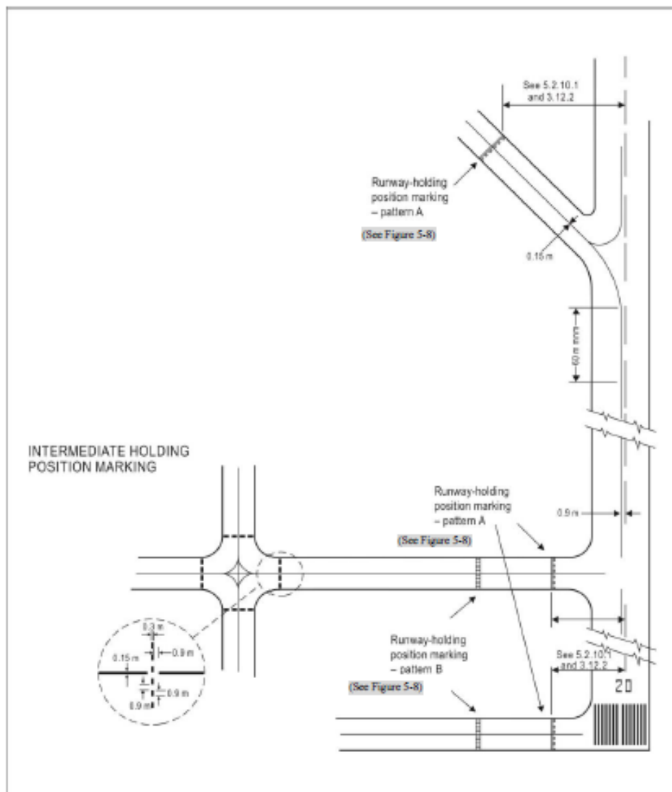
Figure 5-6. Taxiway markings (Shown with basic runway markings)
