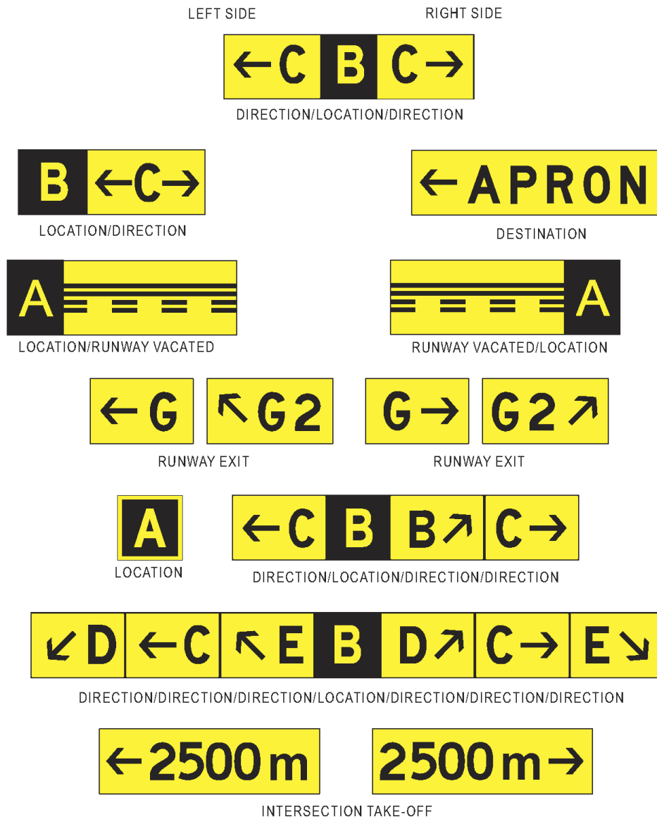
Figure 5-31. Information signs
