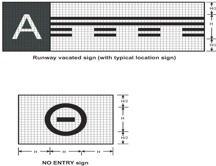
Figure A4-3. Runway vacated and NO ENTRY signs
