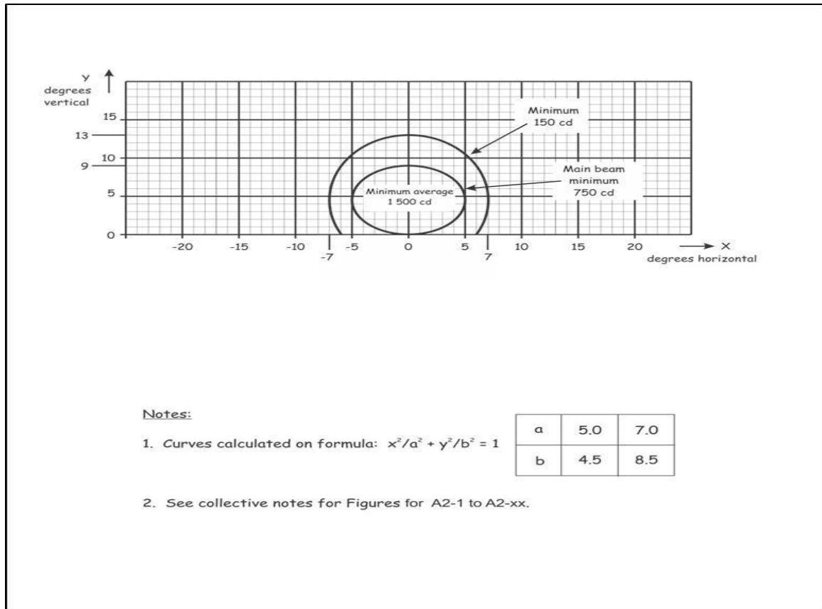
Figure A2-25. Isocandela diagram for each light in high-intensity runway guard lights, Configuration A
