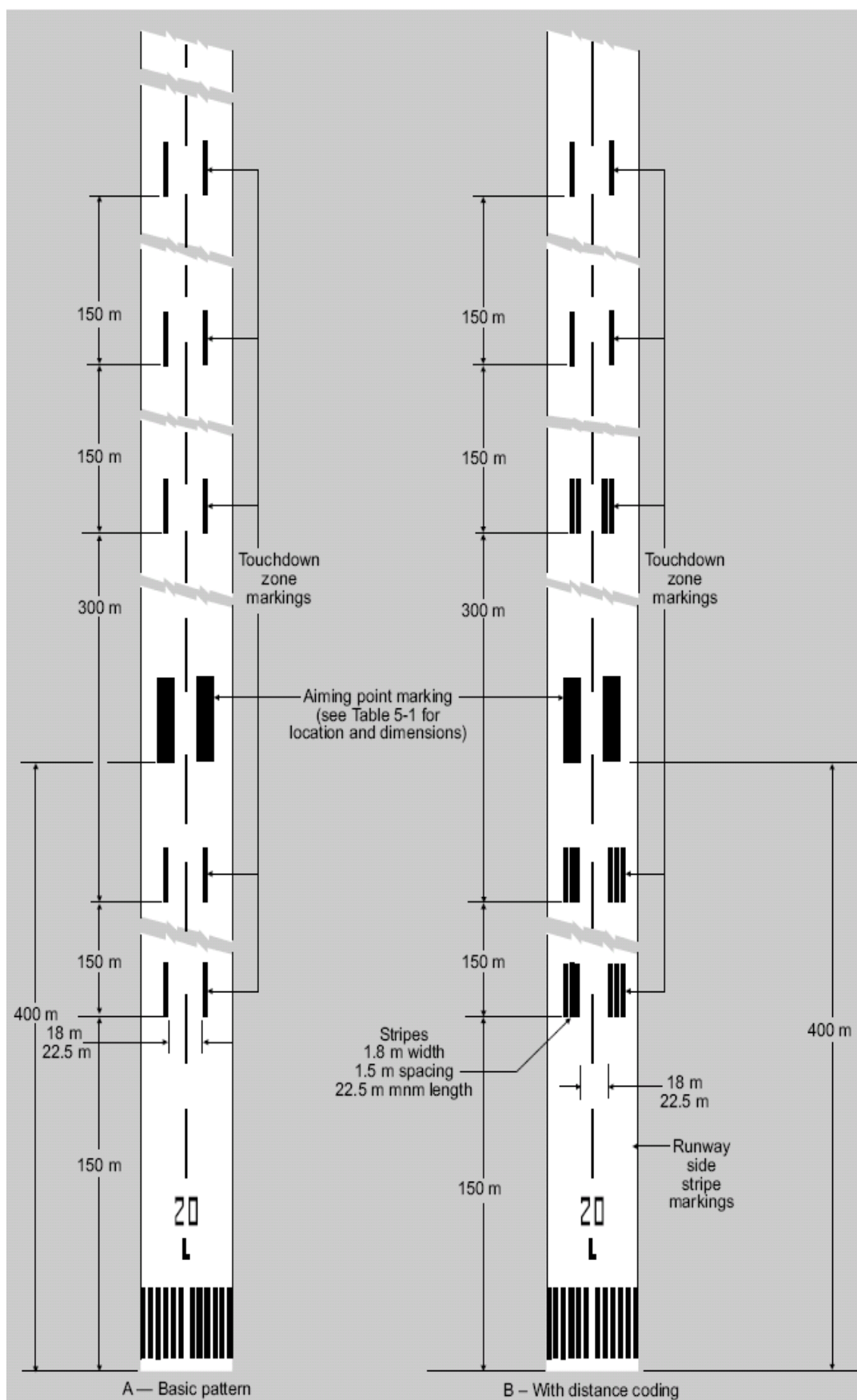
Figure 5-5. Aiming point and touchdown zone markings (illustrated for a runway with a length of 2400 m or more)
