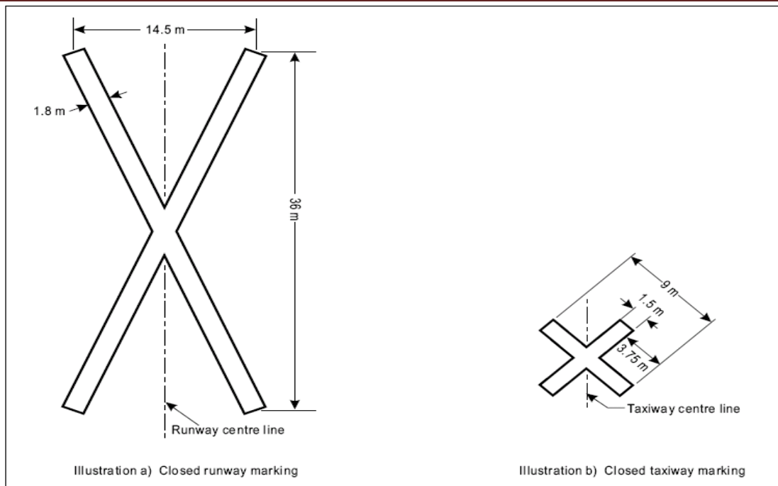
Figure 7-1. Closed runway and taxiway markings
