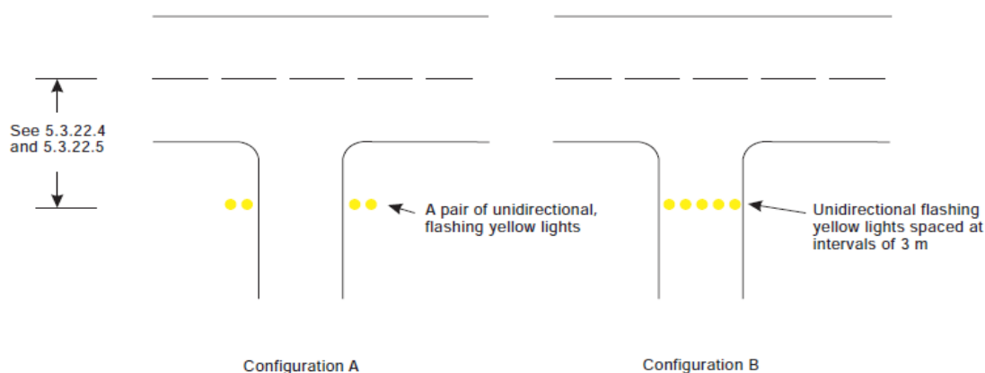
Figure 5-29. Runway guard lights
