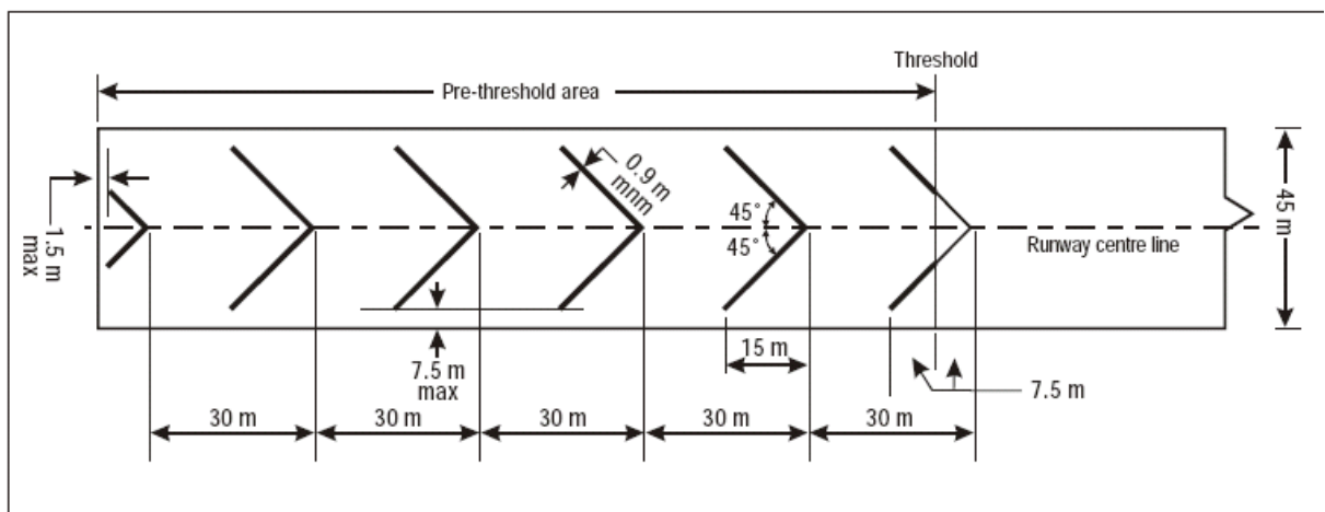
Figure 7-2. Pre-threshold marking
