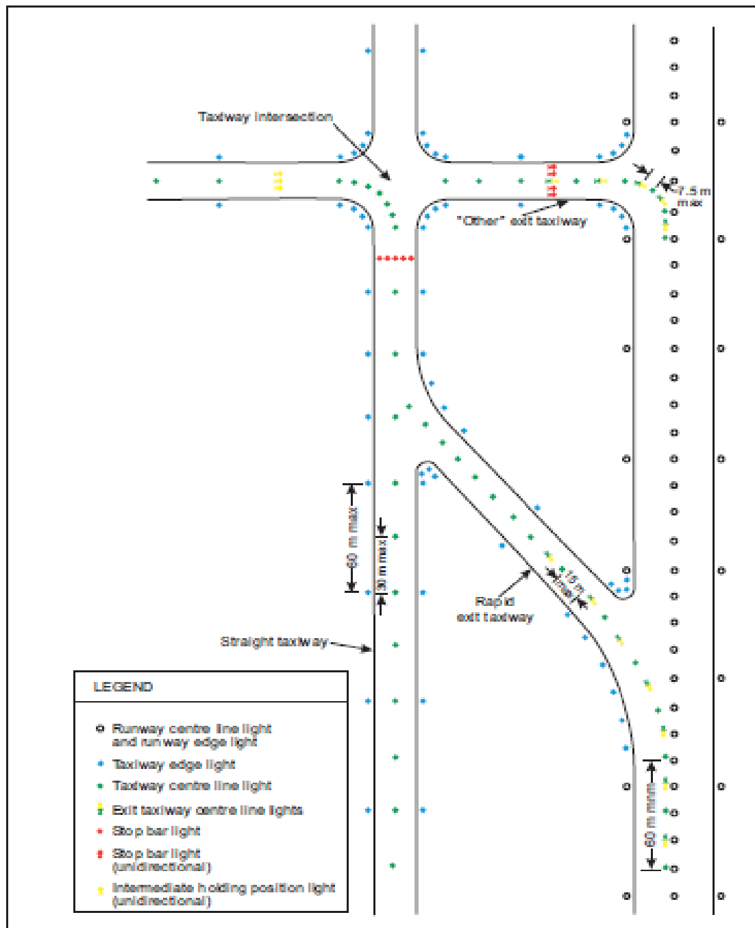
Figure 5-26. Taxiway lighting
