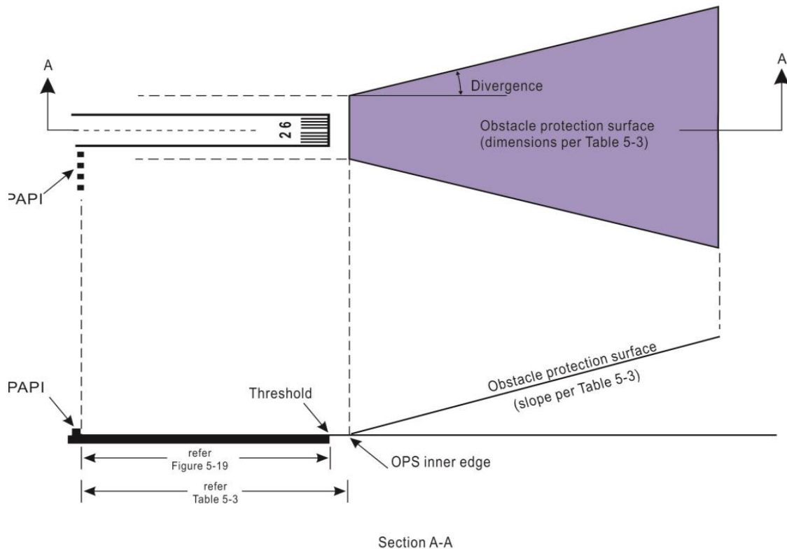
Figure 5-21. Obstacle protection surface for visual approach slope indicator systems
