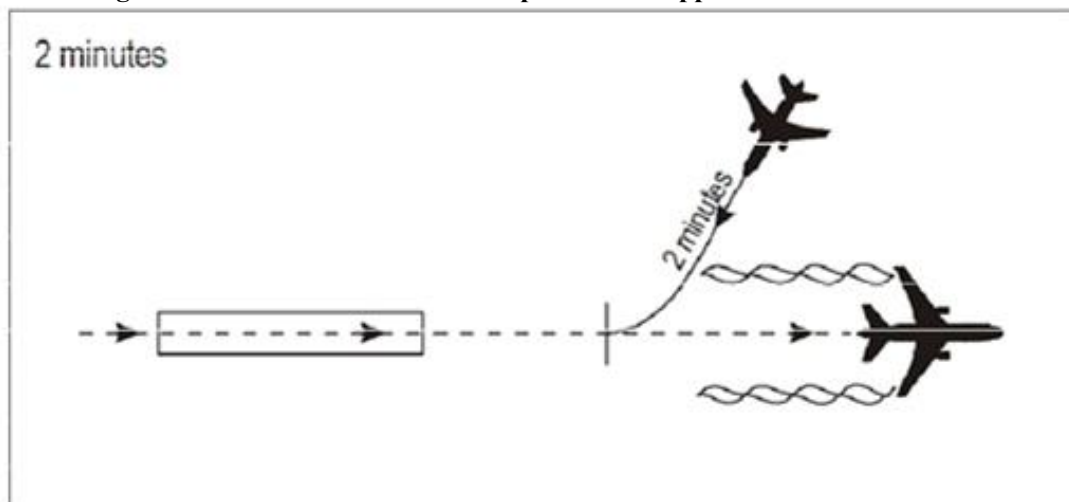
Fig. 5-38. Two Min. wake turbulence separation for opposite direction landing
