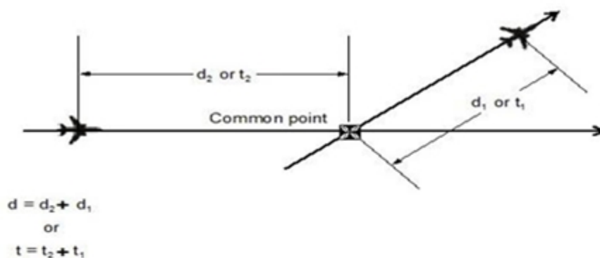
Figure 5-33. Calculation of longitudinal distance/time between aircraft— opposite sides of the common point (see 5.4.2.6.5 b)
