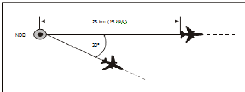
Figure 5.5. Separation using the same NDB (see 5.4.1.2.1.2 b))
