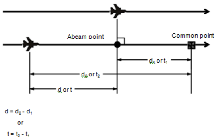
Figure 5-34. Calculation of longitudinal distance/time between aircraft— parallel tracks (see 5.4.2.6.5 c)
