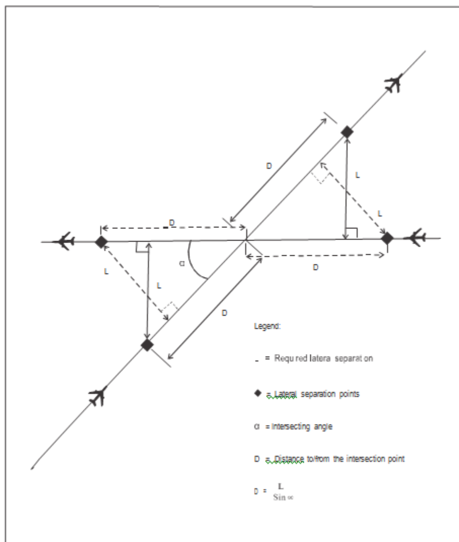
Figure 5-6. Lateral separation points (see 5.4.1.2.1.7)
