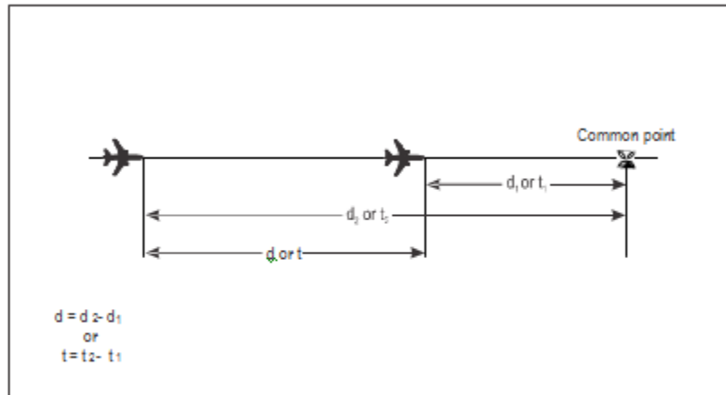
Figure 5-29. Calculation of longitudinal distance/time between aircraft— identical track, same direction (see 5.4.2.6.5 a)
