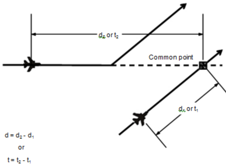
Figure 5-32. Calculation of longitudinal distance/time between aircraft — same track projected, but not identical (see 5.4.2.6.5 b)
