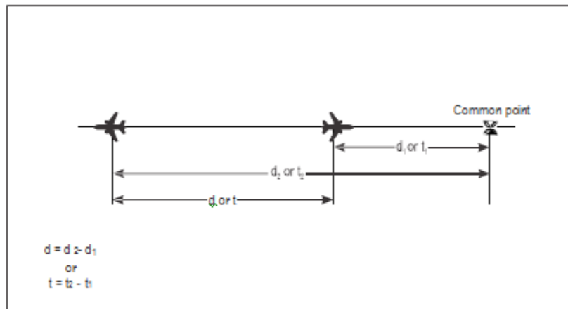
Figure 5-30. Calculation of longitudinal distance/time between aircraft— identical track, opposite direction (see 5.4.2.6.5 a)
