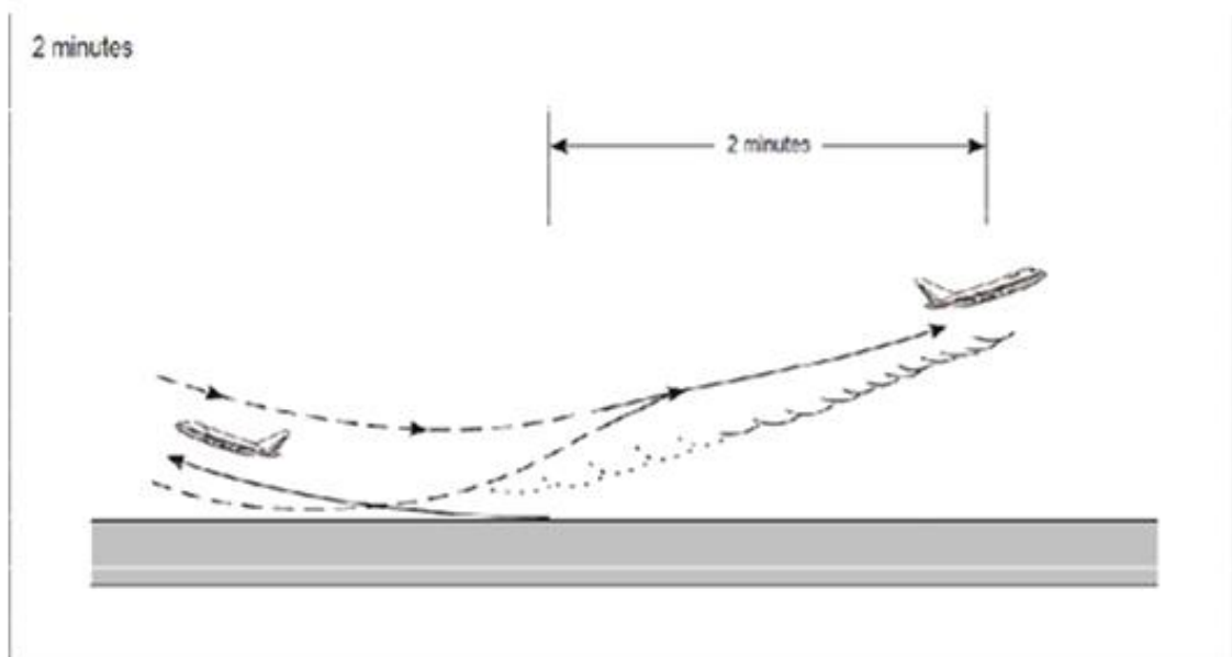
Fig. 37. Two Min. wake turbulence separation for opposite direction take-off
