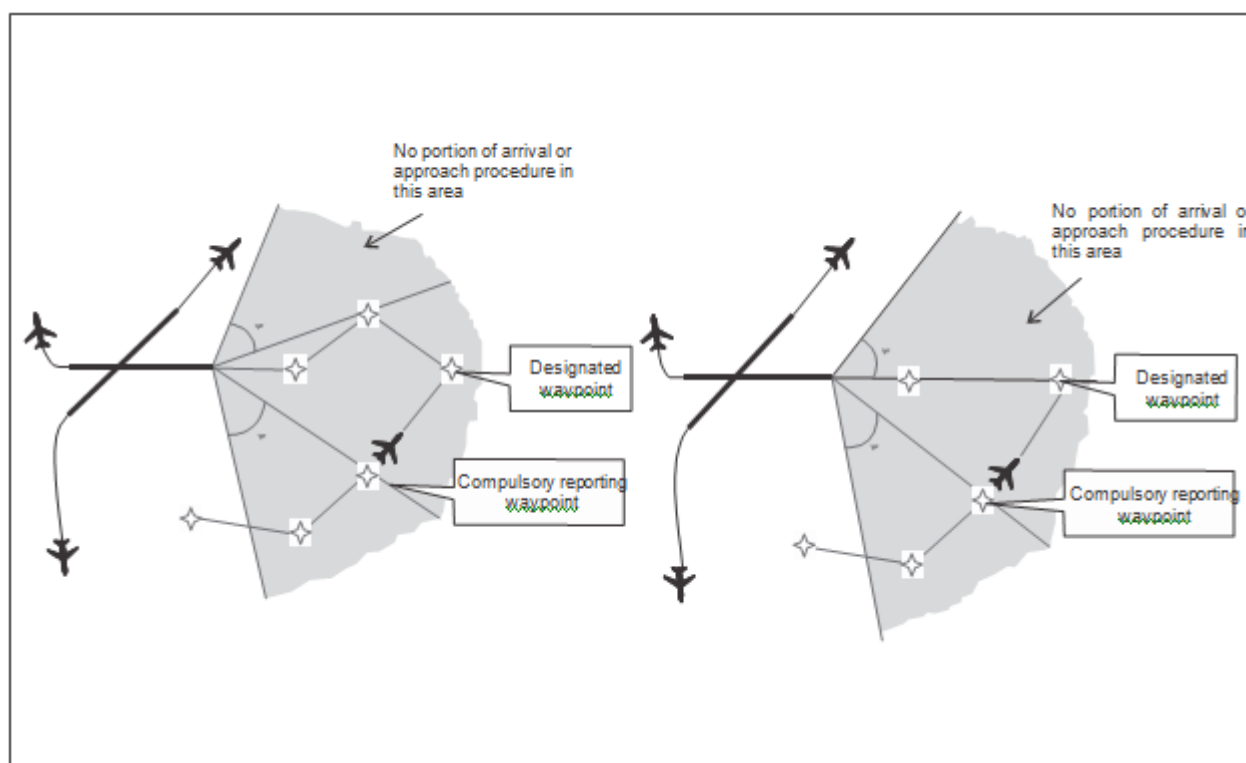
Fig. 5-36. Example of Arrival Protecting Area
