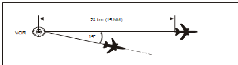
Figure 5.4. Separation using the same VOR (see 5.4.1.2.1.2 a))
