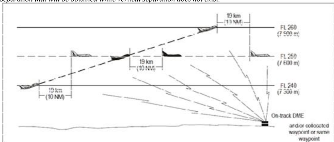
Fig. 5-30A. 10 NM DME and/or GNSS-based separation between aircraft climbing and on same track
