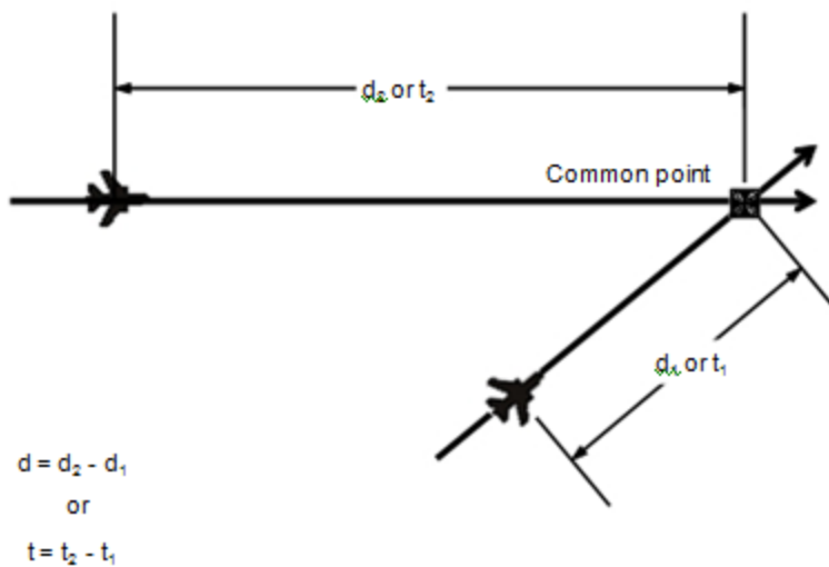
Figure 5-31. Calculation of longitudinal distance/time between aircraft — same track, but not identical and crossing tracks (see 5.4.2.6.5 b)
