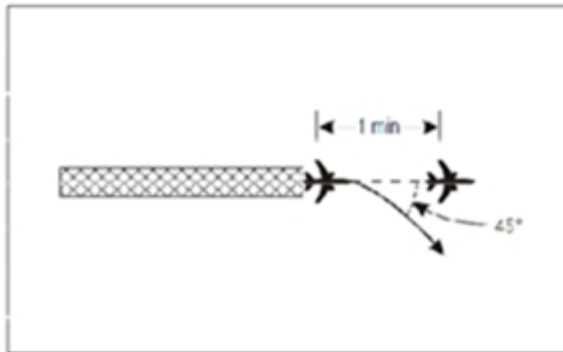
Fig. 5-32. One Min. separation between departing aircraft following tracks diverging by at least 45 degrees
